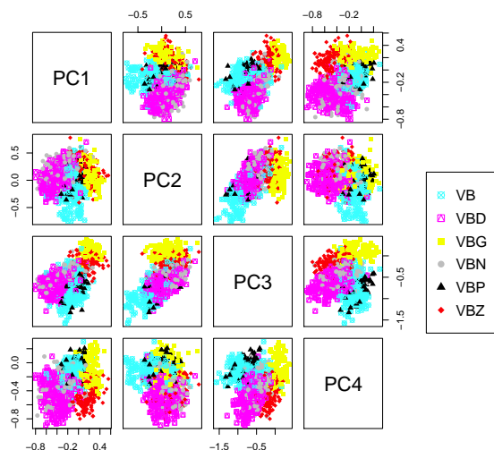
(b) PCA of the hidden activations of L_p(p = 2)
